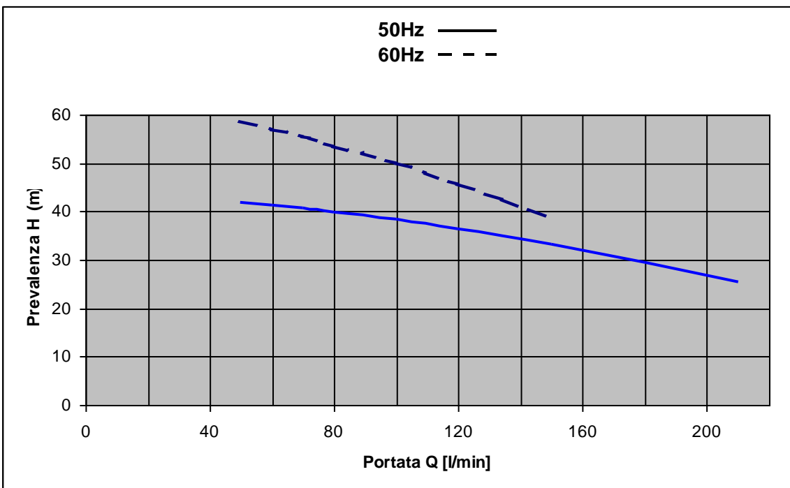
WRAC8-D8 centrifuge pump at 50-60Hz: WLAC8-D8 centrifuge pump at 50-60Hz:
